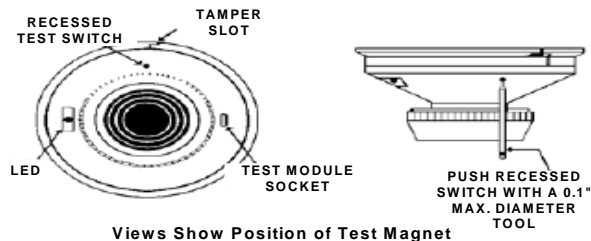
Views Show Position of Test Magnet
