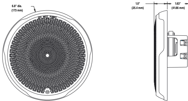
Ceiling-Mount Speaker
