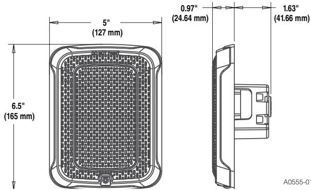
Wall-Mount Speaker
