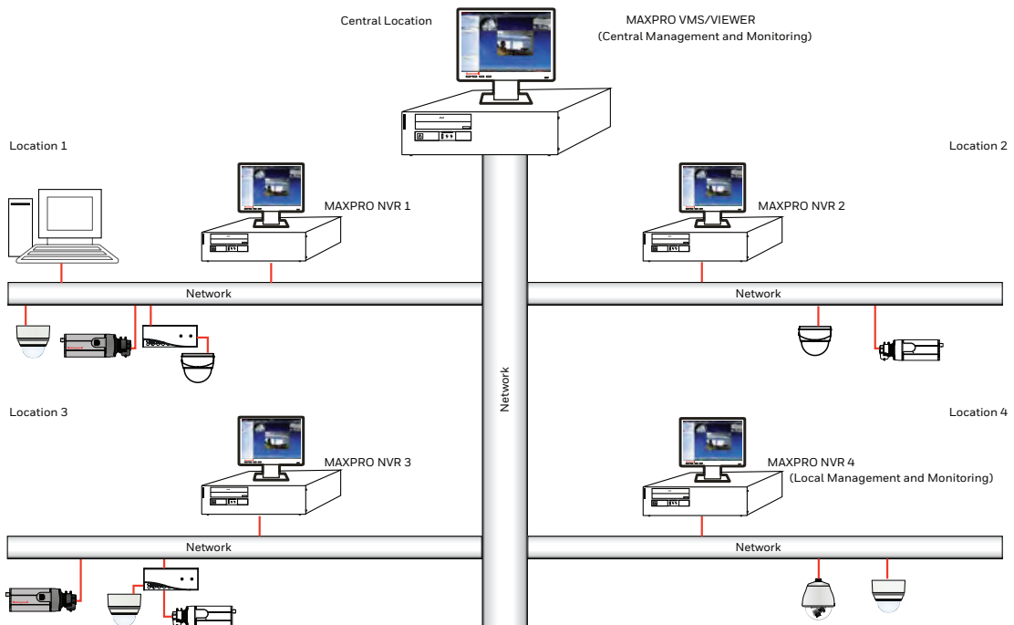
MAXPRO NVR Multiple NVRs – Distributed Architecture
