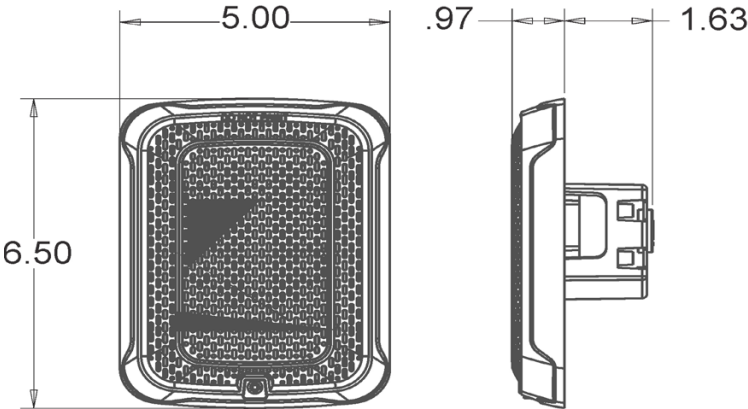
WALL-MOUNT SPEAKER
