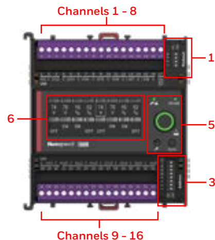
16 Universal I/O with HOA
