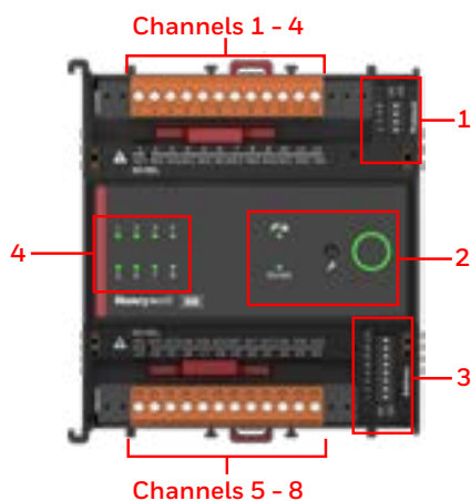
8 Digital Outputs
