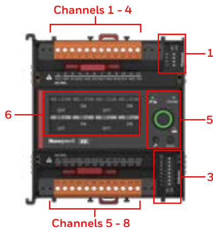
8 Digital Outputs with HOA
