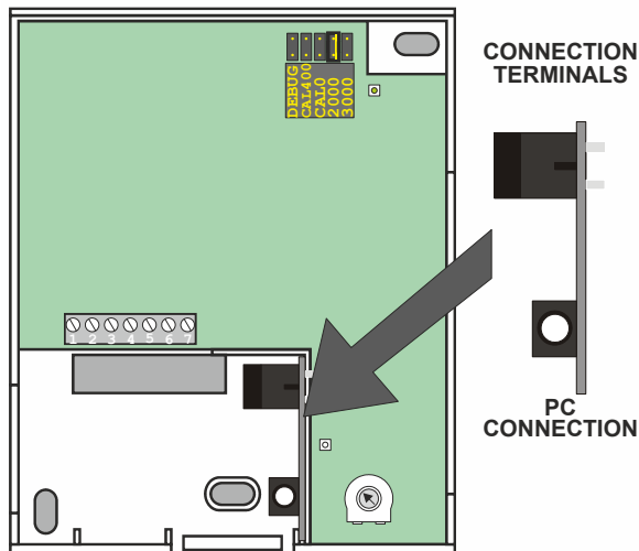
Fig. 14. Mounting the T7460-LONJACK
