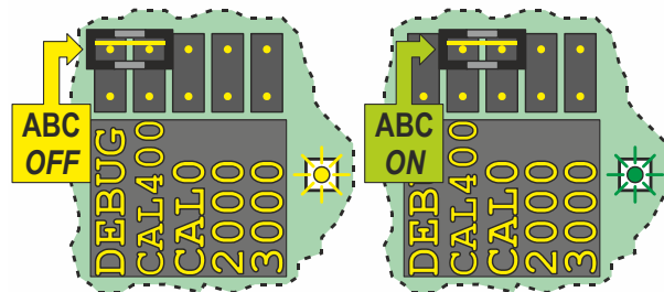
Fig. 9. Switching ABC OFF (left) or ON (right)
