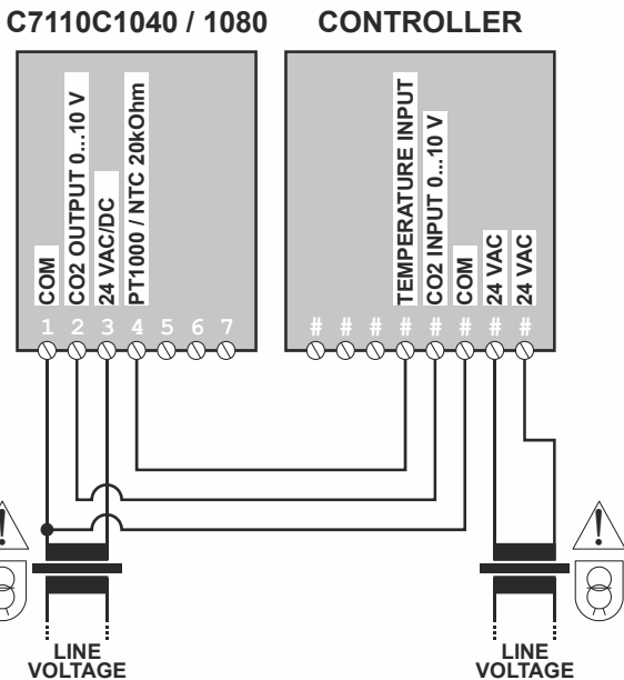
Fig. 4. Wiring C7110C1040 / 1080 to controller and separate safety transformer
