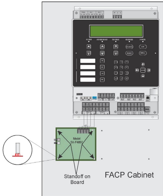
SK-F485C MOUNTING IN FACP CABINET
