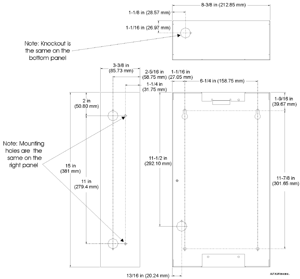
Backbox Dimensions
