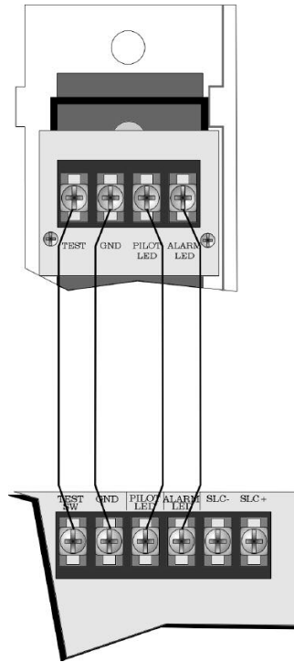
DTS-K Connection
