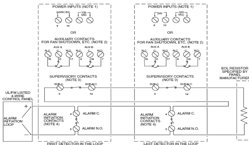
Figure 4 Wiring for 4-Wire Duct Smoke Detector and Accessories
