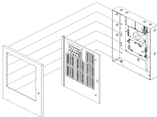
Figure 2 FCI 7200 CAB-C Configuration
