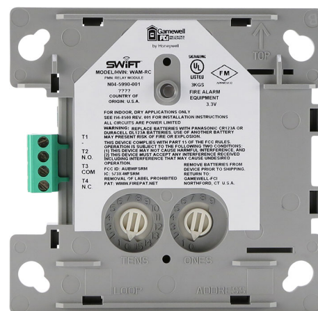
WAM-RC Wireless Relay Module
