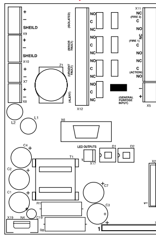
Detector Termination Card 7 Relay Version
