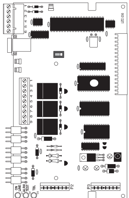
UZY-256 Universal Zone Coder
