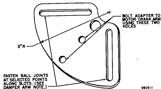
Fig. 1 — Approximate Dimensions of Linkage Components.
