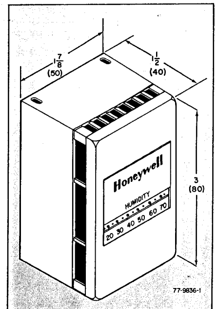
FIG. 3. ALL COVERS—VERTICAL OR HORIZONTAL, STANDARD OR NO-DISPLAY—ARE THE SAME SIZE; APPROXIMATE DIMENSIONS ARE GIVEN IN INCHES (AND MILLIMETERS).
