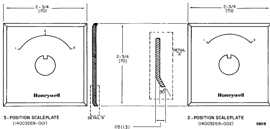
Fig. 2. Approximate Dimensions of Scaleplate in Inches (Millimeters).
