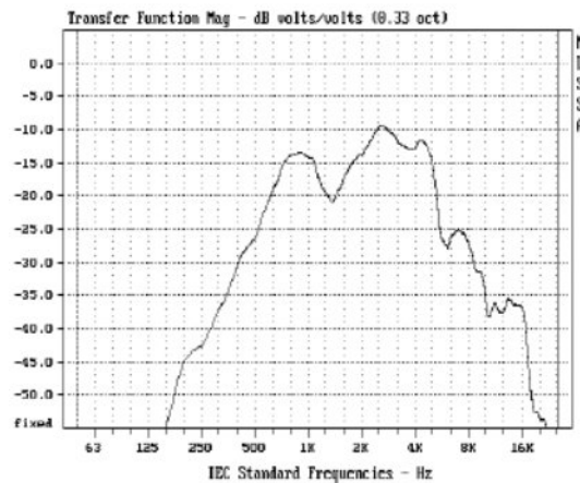
Wall Speaker Strobe Wide Band Frequency Response
