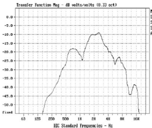
Ceiling Speaker Strobe Wide Band Frequency Response
