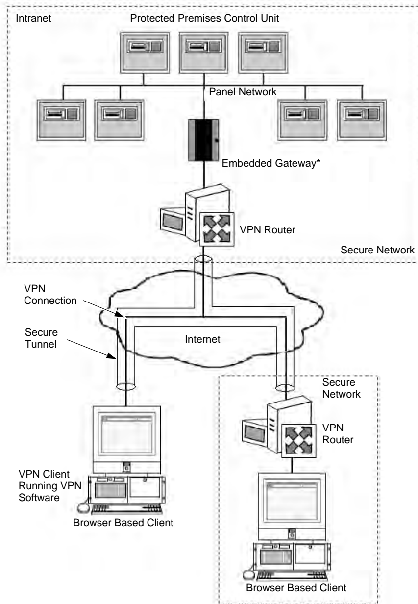
Figure 2.3 Embedded Gateway VPN Setup
