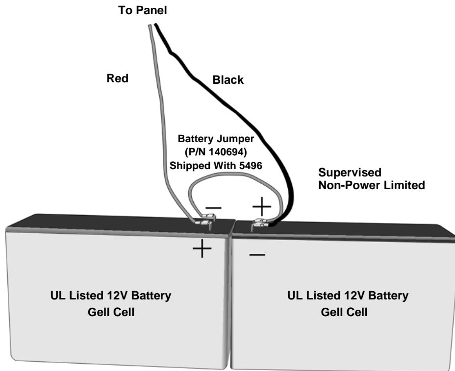
Figure 3-2 Battery Connection
