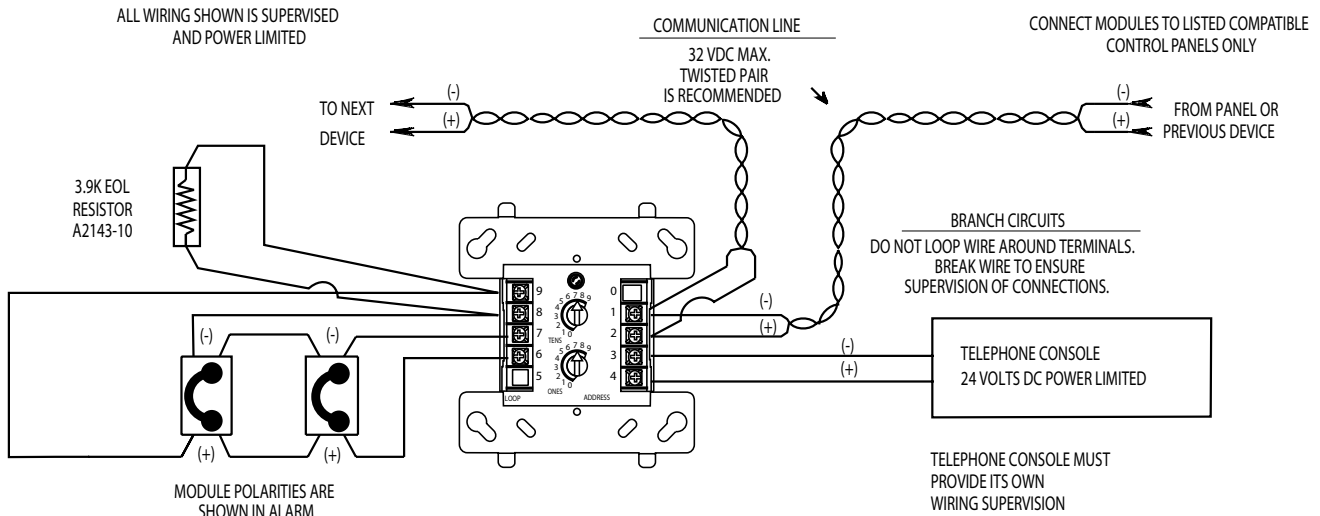
Figure 4. Typical fault tolerant circuit configuration, NFPA Style Z, Class A style wiring:
