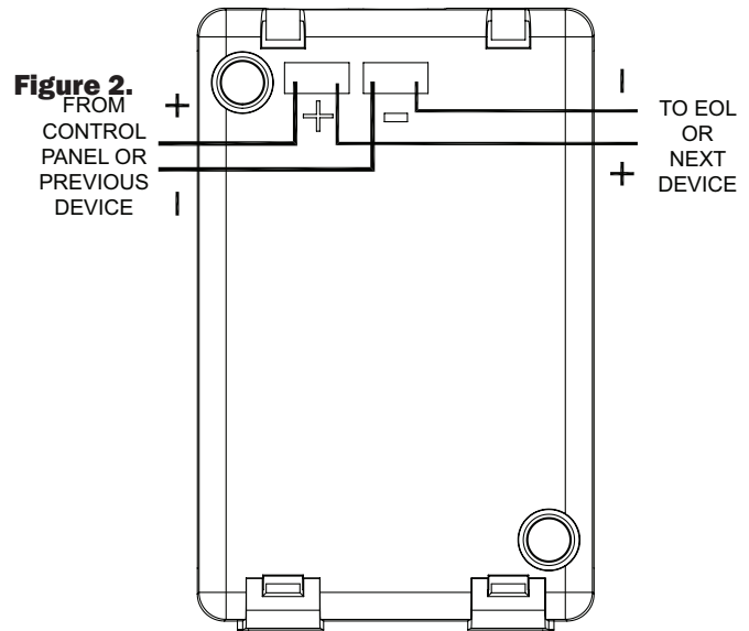
NOTE: SHOWN WITH CONTROL PANEL IN ALARM. PANEL POLARITY REVERSED IN SUPERVISORY CONDITION. A0358-00
