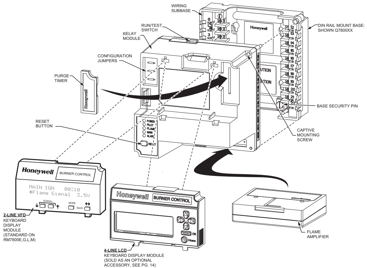
Fig. 5. RM7800/RM7840 Relay Module exploded view.
