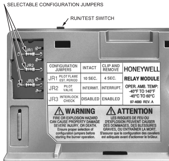
Fig. 6. Selectable site-configurable jumpers.
