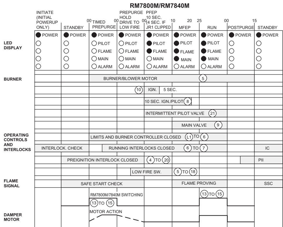
Fig. 4. Wiring subbase and sequence for RM7800M/RM7840M.
