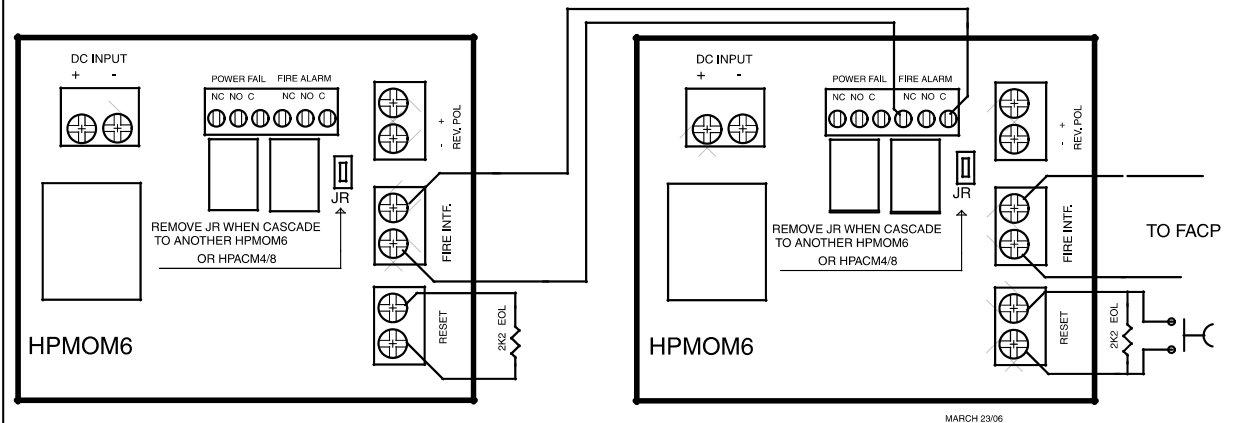
FIG.1a CONNECTION OF TWO (2) OR MORE HPMOM6 OR HPACM4/8
