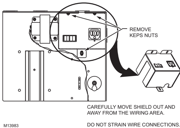
Fig. 5. Power wiring shield for ENC-H-001 or -002 enclosure
