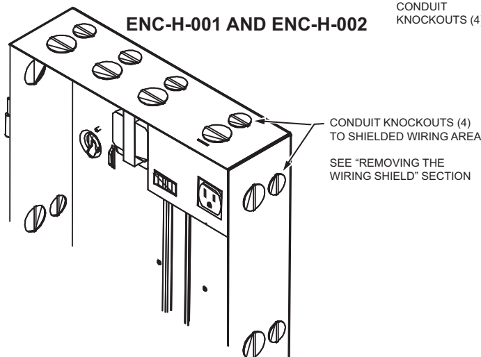
Fig. 1. Knockout numbers and locations for ENC-H-001 and ENC-H-002 enclosures.
