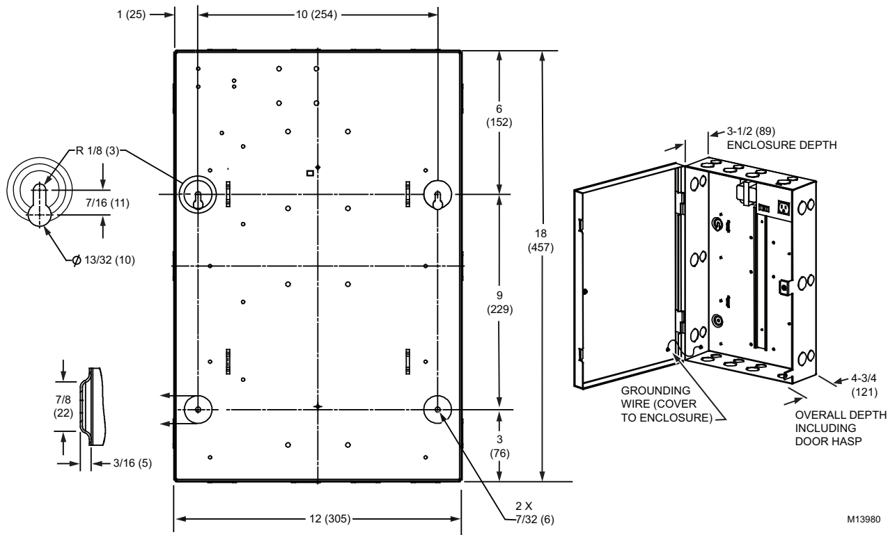
Fig. 2. ENC-H-001 enclosure wall mounting details.
