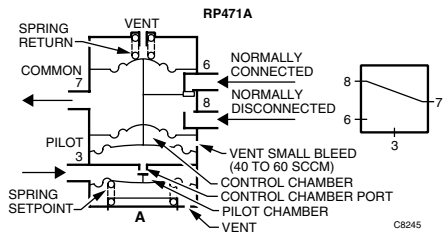
Fig. 5. RP471A operation.
