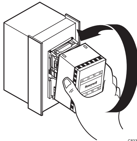
Fig. 4. Mounting cover
