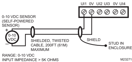
Fig. 6. 0-10 Vdc wiring.
