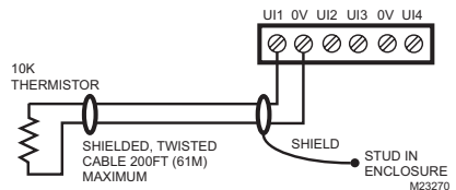
Fig. 5. Thermistor wiring.
