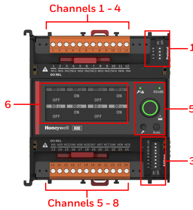
8 Digital Outputs with HOA
