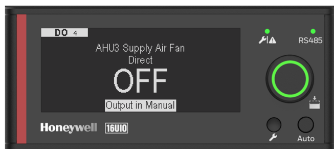
Fig. 17. Channel Screen in Manual Mode
