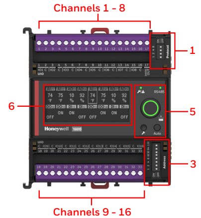
16 Universal I/O with HOA
