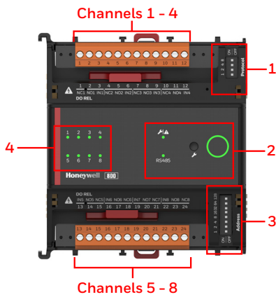
8 Digital Outputs
