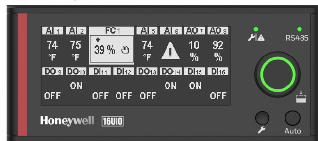
Fig. 19. FC - Side by side Configuration
