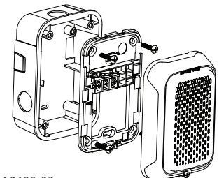
FIGURE 8. SURFACE MOUNT BACK BOX UP ARROW
