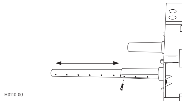
Figure 2. Plastic sampling tube connected to duct smoke detector:
