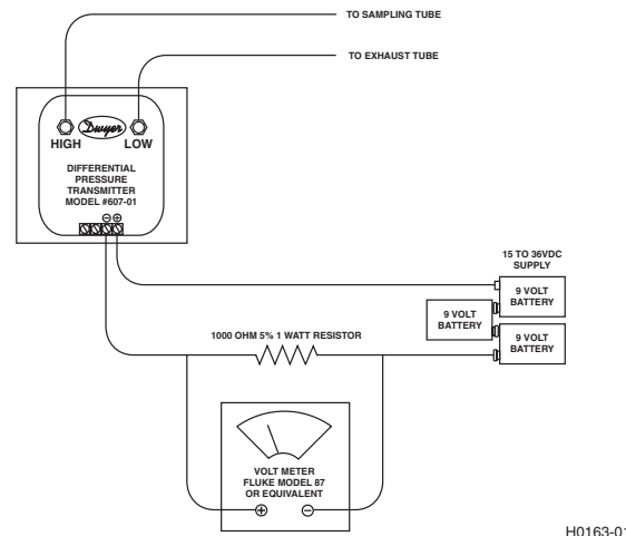
Figure 8. Procedure for verifying air flow:
