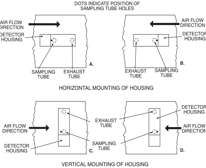
Figure 5. Tube mounting configurations with varying air flow direction:
