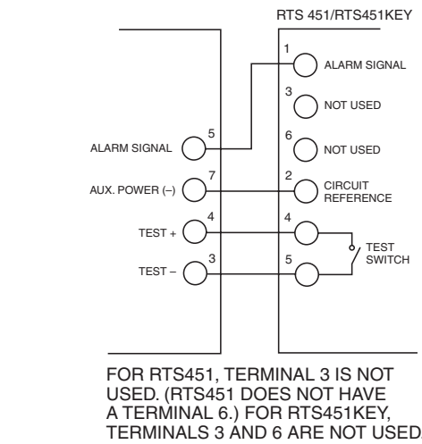
Figure 11. System Wiring Diagram for DH200RPL Duct Smoke Detector with RTS451/RTS451KEY:
