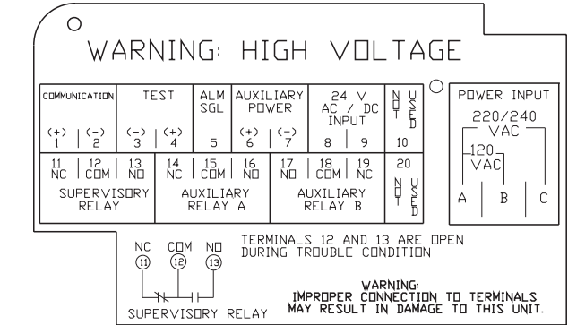
Figure 14. Insulator Card for DH200RPL Duct Smoke Detector:
