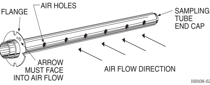
Figure 4. Air duct detector sampling tube:
