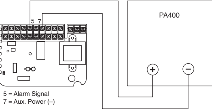
Figure 12. Wiring Diagram for DH200RPL with optional PA400:
