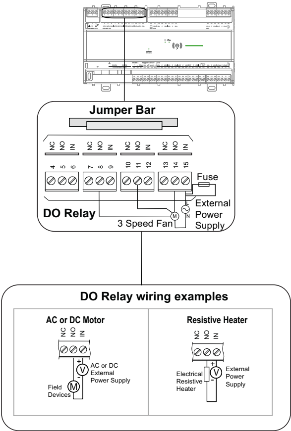
Fig. 20 SPDT Relay Wiring Examples
