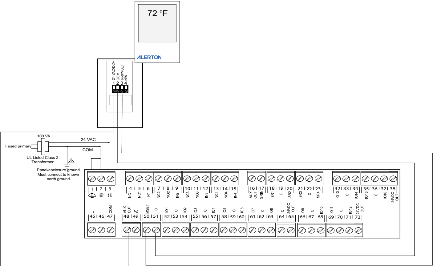
Fig. 21 Alerton Unitary Controller wiring with MS4
