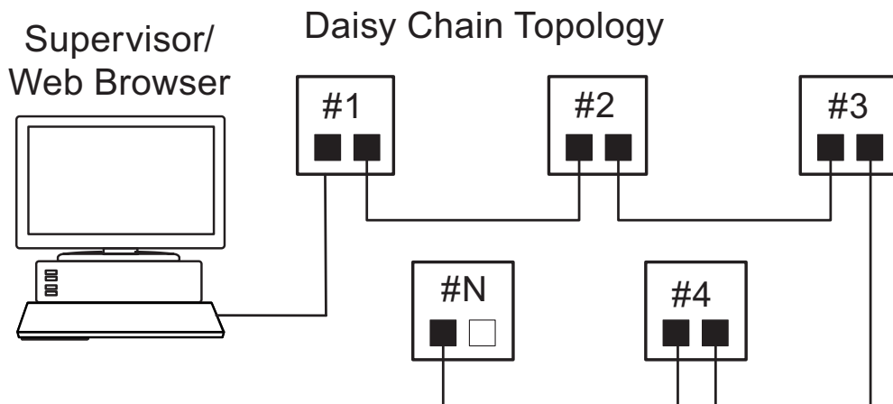
Fig. 57 Daisy chain topology
