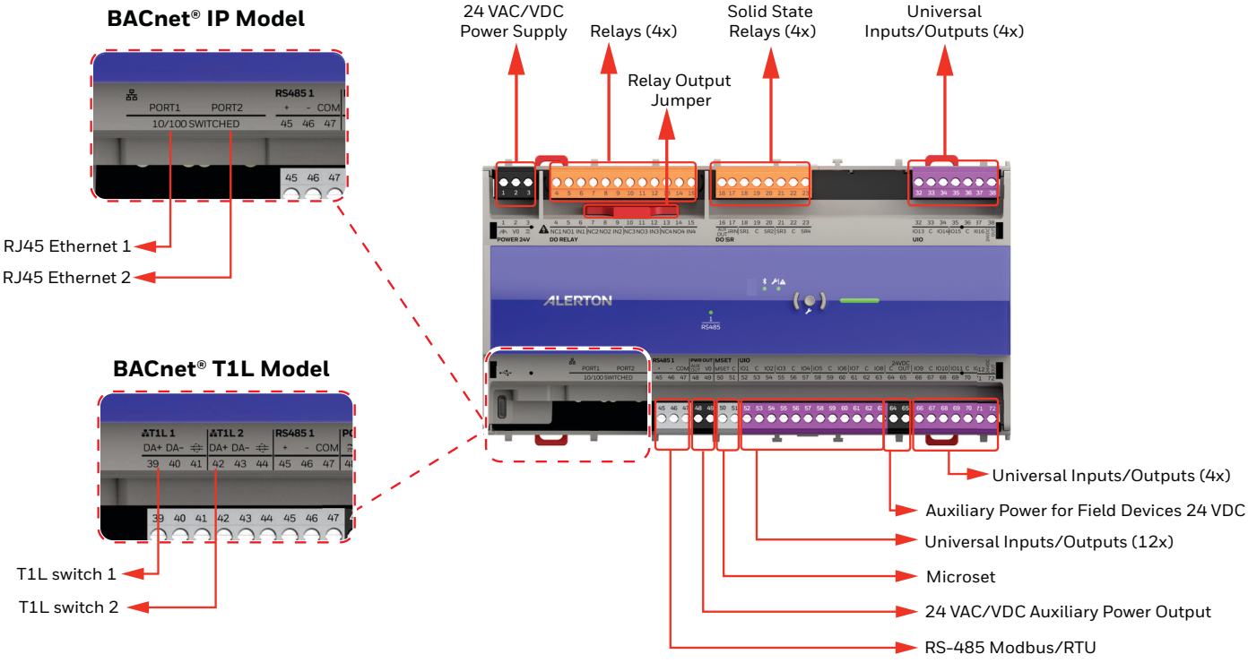
Fig. 4 Unitary Controllers (Large) Overview
