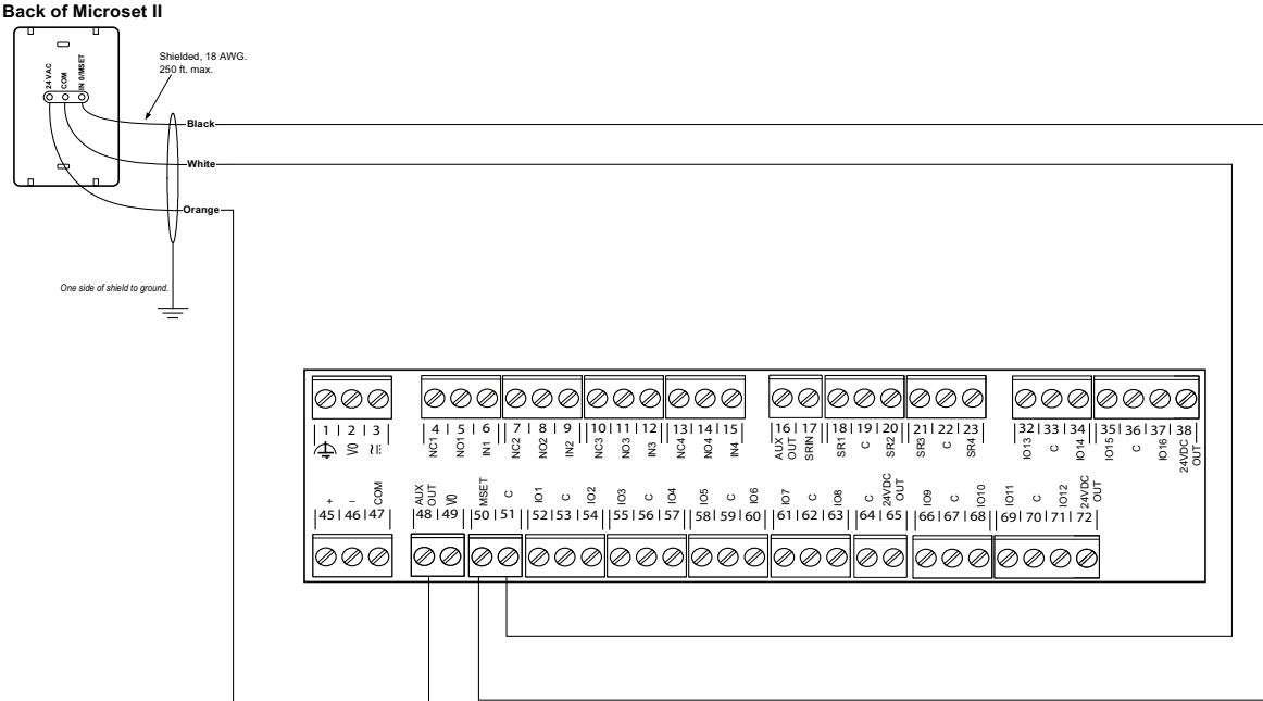
Fig. 22 Alerton Unitary Controller wiring with MS2
