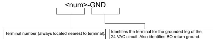
Fig. 13 Grounded terminals
