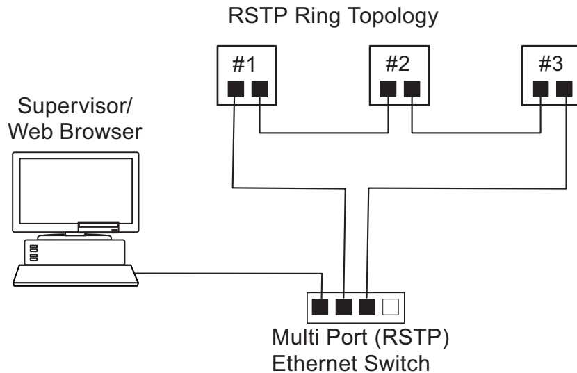
Fig. 58 Ring Topology
