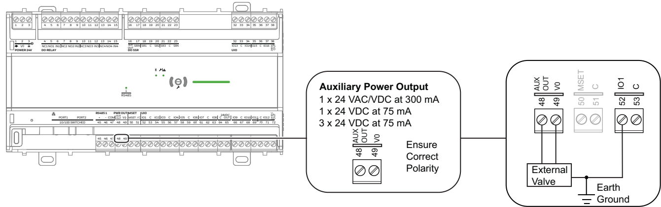
Fig. 19 Auxiliary Wiring Examples
