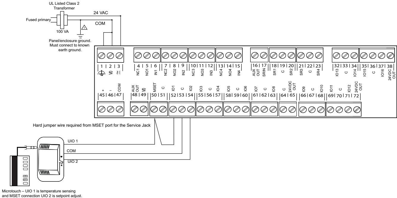
Fig. 23 Alerton Unitary Controller wiring with Microtouch
