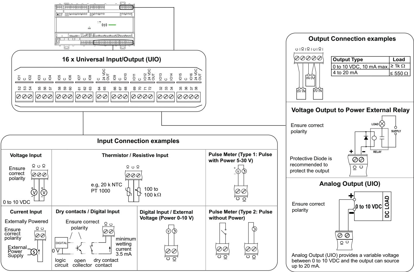
Fig. 17 Universal IO Wiring Examples
