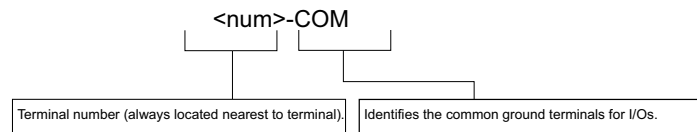
Fig. 14 Common terminals
