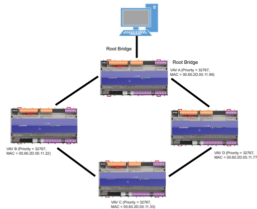
Fig. 61 Root Bridge Example 2
