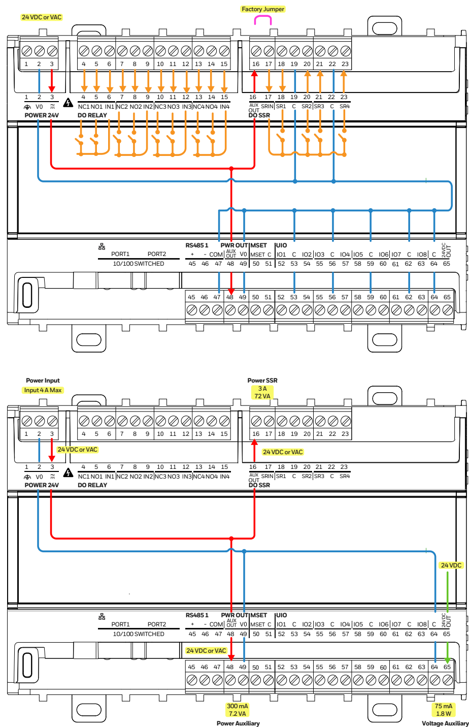
Fig. 11 Internal Wiring Small controller
