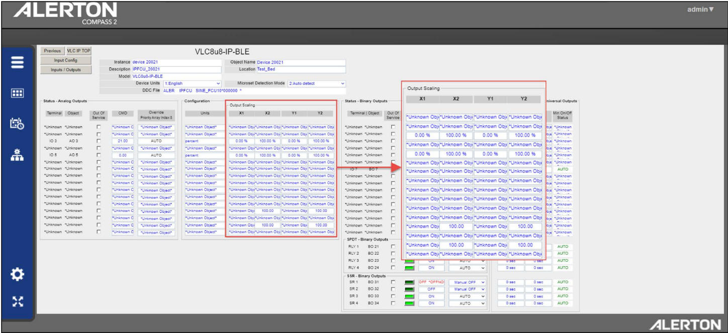
Fig. 53 Output scaling
