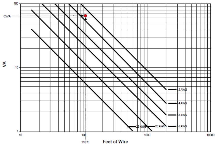
Fig. 8 Example of determining appropriate wire type
