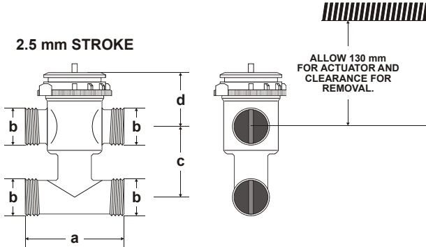
Fig. 6. VSxC-4 / VSxF-4 (3-way with bypass + snap-on), dimensions
