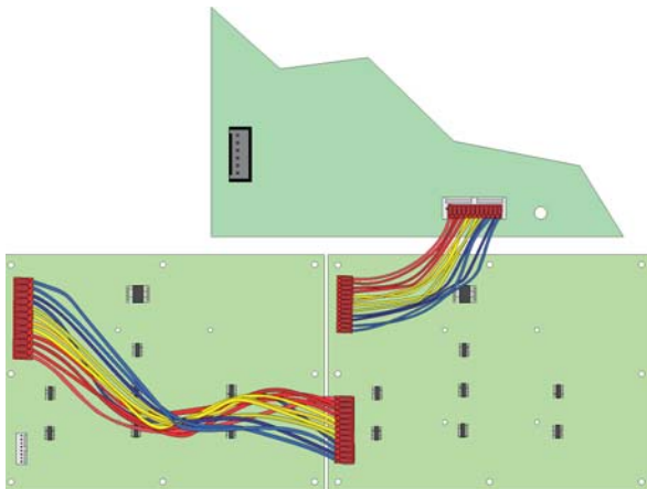
Figure 4: Wiring Harness Connection for IFP-2000ECS
