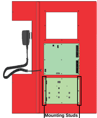
Figure 1: IFP-1000ECS and IFP-100ECS Mounting Location for the ECS-SW24
