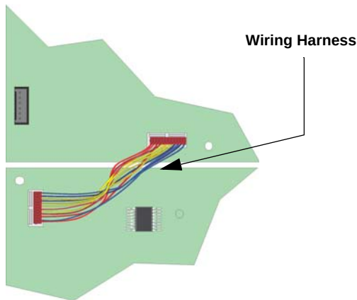
Figure 3: Wiring Harness Connection for the IFP-100ECS and IFP-1000ECS
