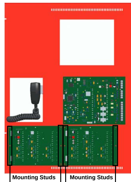
Figure 2: IFP-2000ECS Mounting Location for the ECS-SW24
