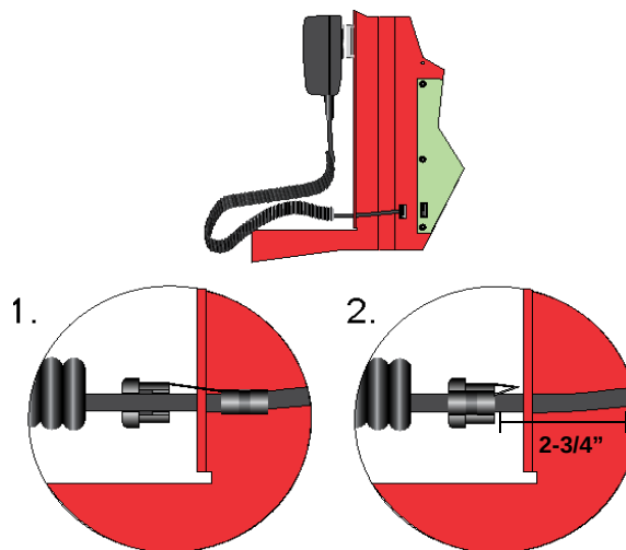
Figure 5: Installing Strain Relief Clip
