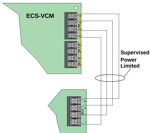
Figure 2: Wiring the ECS-VCM to the FACP
