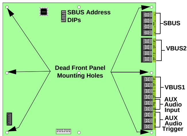
Figure 1: Back View of ECS-VCM
