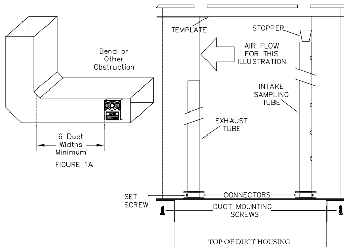
FIGURE 1B: DUCT HOUSING MOUNTING
