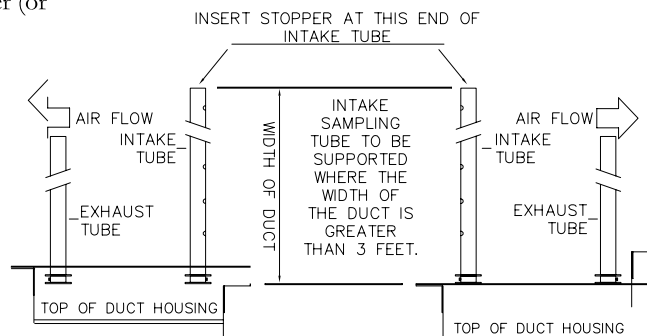
FIGURE 2 SAMPLING TUBE ORIENTATION
