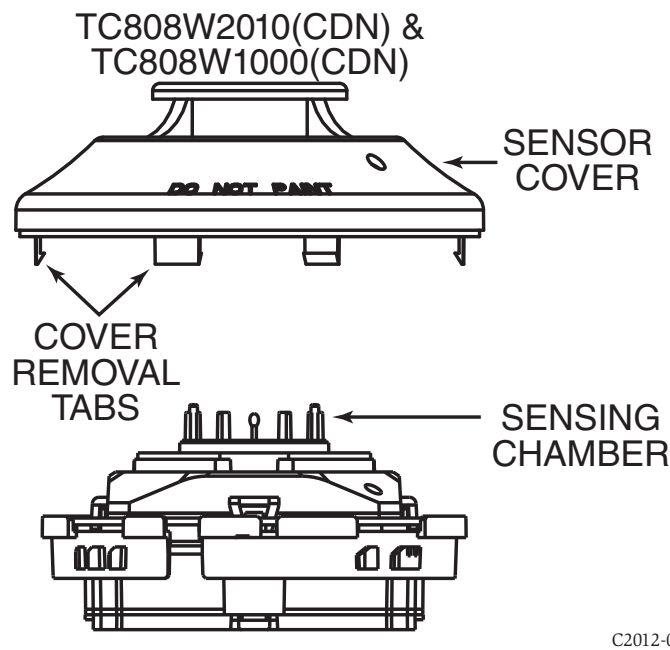
FIGURE 5. DETECTOR COMPONENTS
