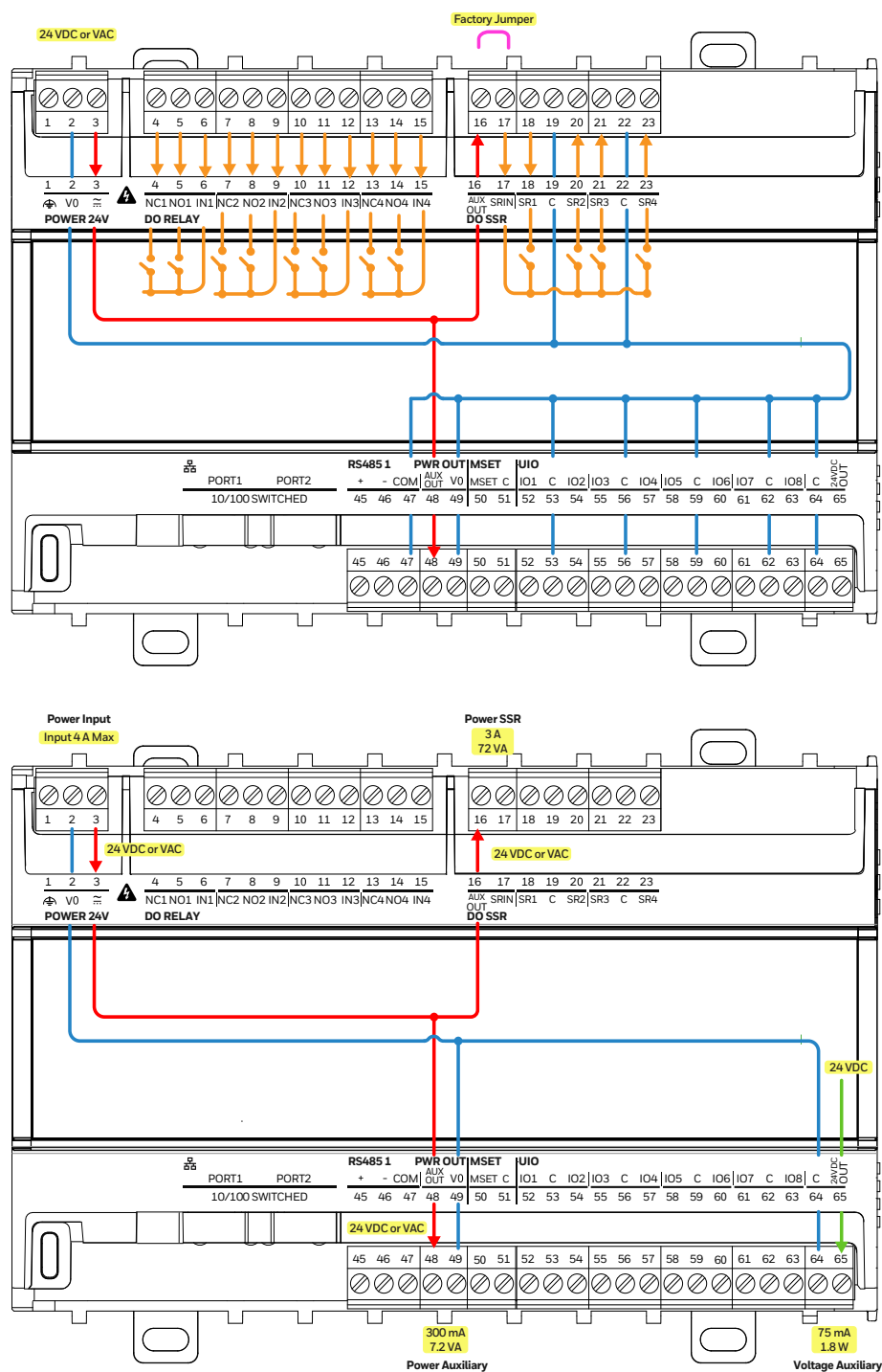
Fig. 12 Internal Wiring Small controller
