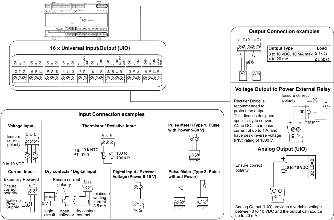
Fig. 18 Universal IO Wiring Examples
