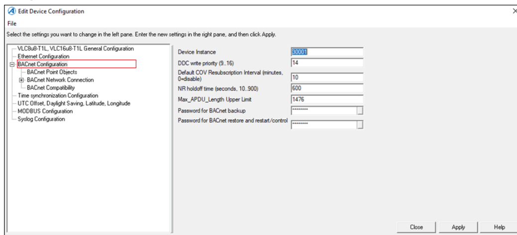
Fig. 31 BACnet Configuration
