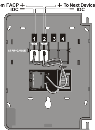
Dual Action NBG-12, 12L 12LSP Wiring
