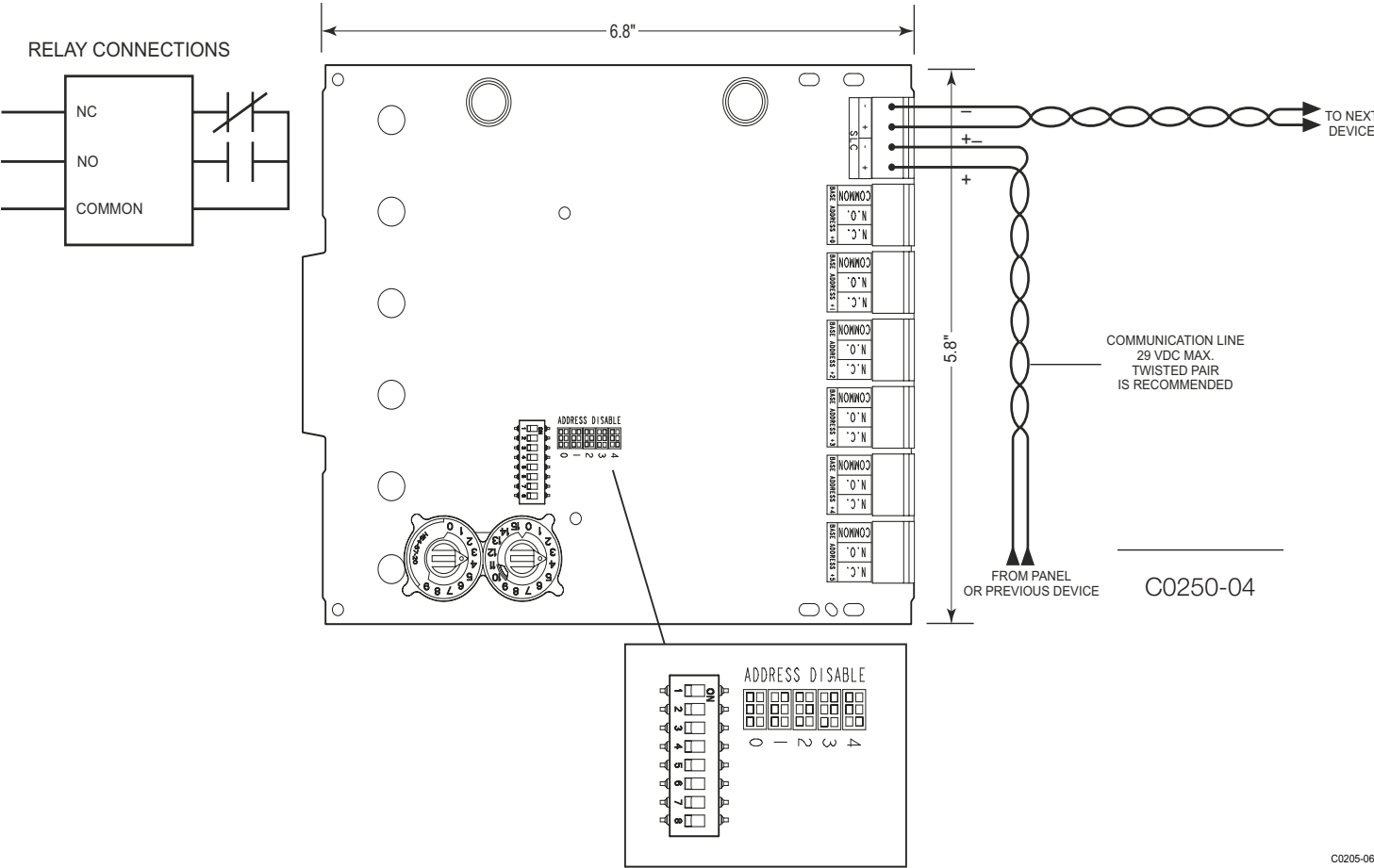
FIGURE 7. WIRING AND PROGRAMMING THE CRF-300-6 MODULE:
