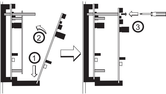
FIGURE 6B. INSTALLATION OF CRF-300-6 MODULE IN FRONT CHASSIS POSITION:
