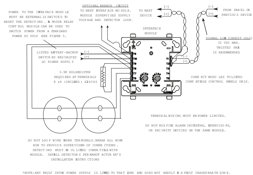
FIGURE 4. INTERFACE TWO-WIRE CONVENTIONAL DETECTORS, NFPA CLASS A
