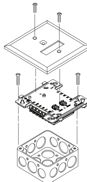
FIGURE 3. INTERFACE TWO-WIRE CONVENTIONAL DETECTORS, NFPA CLASS B
