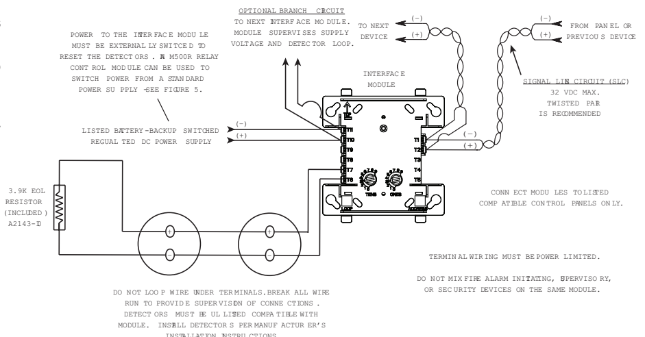
FIGURE 3. INTERFACE TWO-WIRE CONVENTIONAL DETECTORS, NFPA CLASS B
