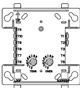
FIGURE 1. CONTROLS AND INDICATORS
