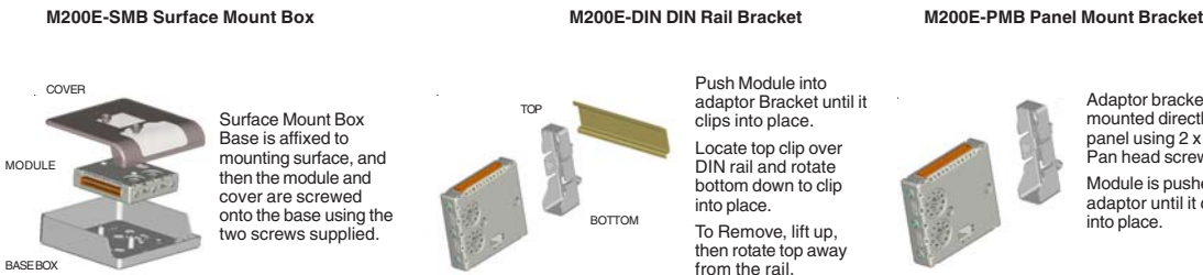
FIGURE 1: MODULE MOUNTING METHODS
