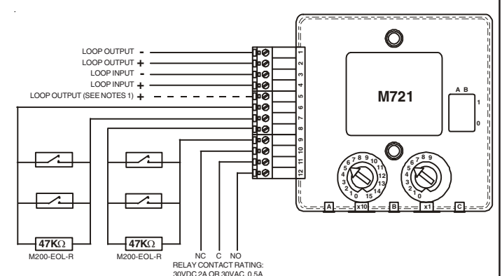
FIGURE 4: M721 DUAL INPUT SINGLE OUTPUT MODULE WIRING
