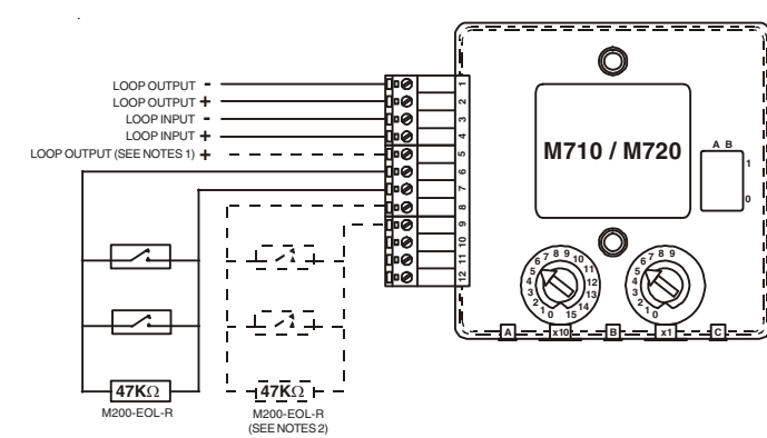
FIGURE 3: M710 SINGLE INPUT AND M720 DUAL INPUT MODULE WIRING
