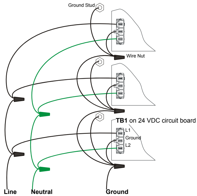
Figure 2.19 Power-Limited Wiring Example: EQBB-D4 AC Wiring (Expanded)
