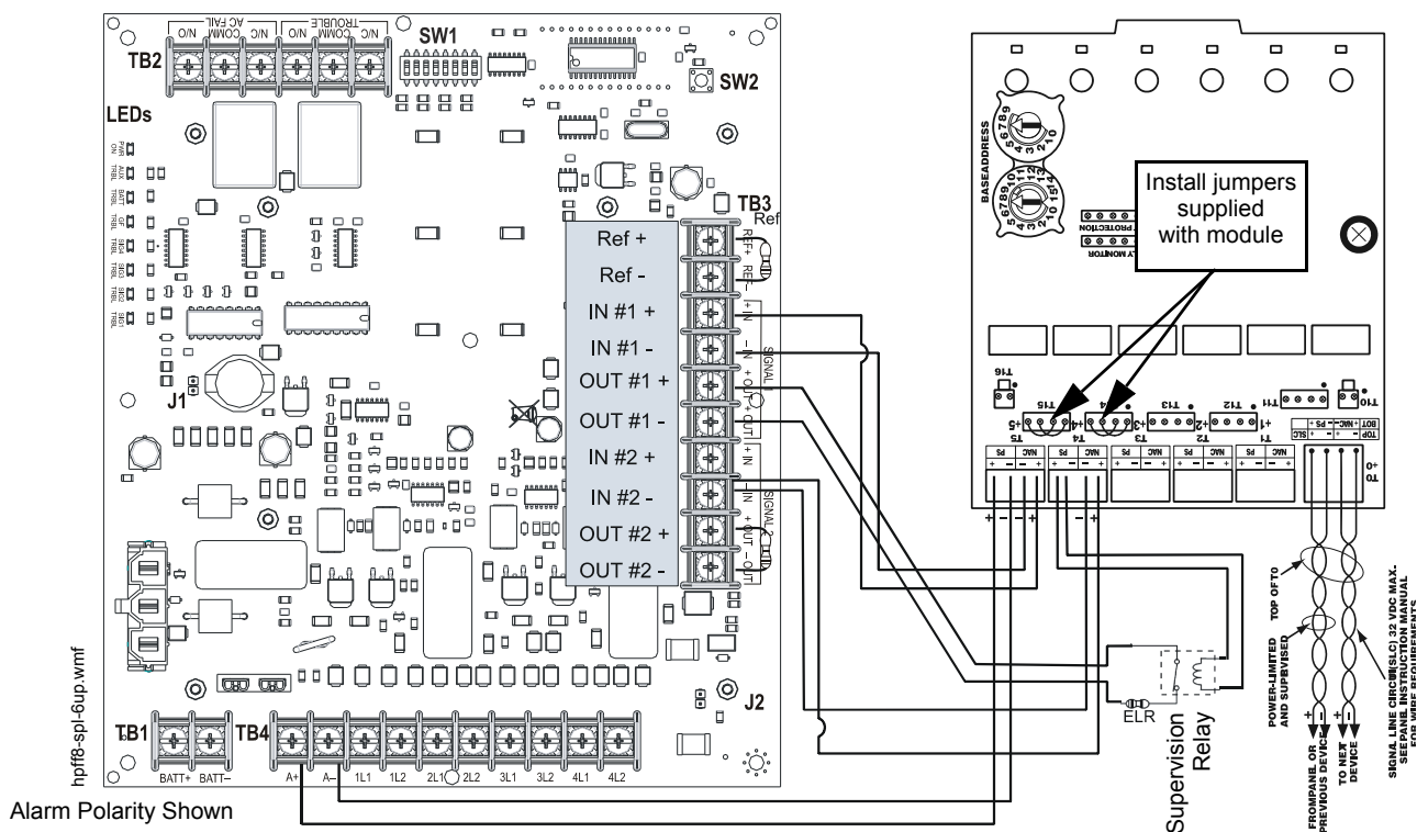
Figure 5.4 Wiring for Split Alarm Mode
