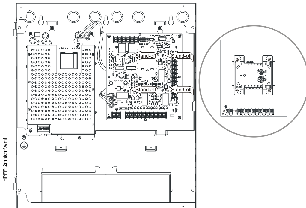
Figure 2.14 Mounting Details for Control & Relay Modules from Honeywell Fire Systems
