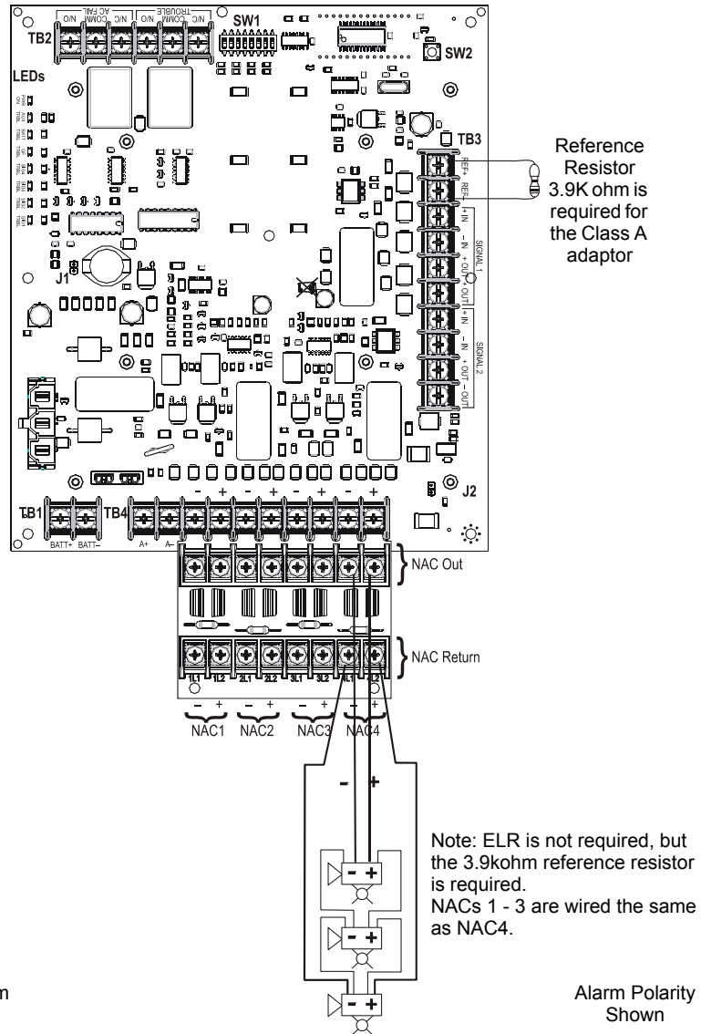
Figure 2.13 Four Class A (Style Z) NACs with HPP31076 Adaptor
