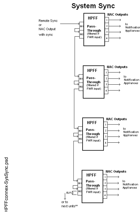
Figure 5.6 System Sync Connections
