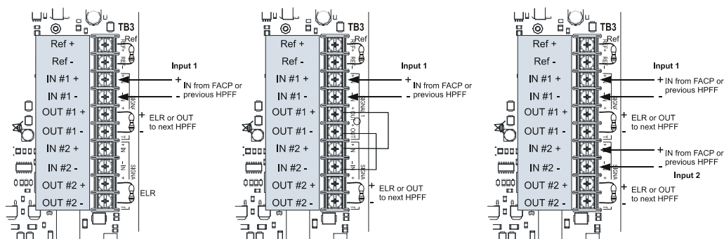
Figure 5.7 Class B Input Connections
