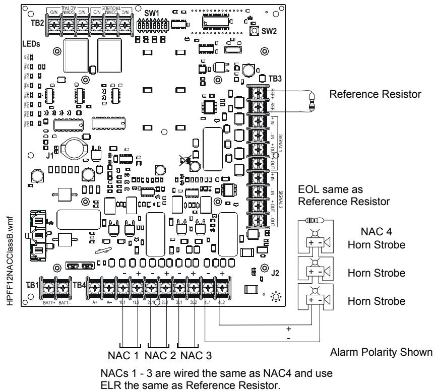
Figure 2.10 Four NACs in Class B (Style Y)
