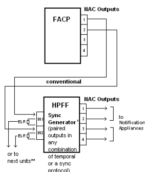
Figure 5.9 Split Alarm Connections
