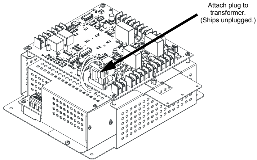
Figure 2.5 Attaching Transformer Plug
