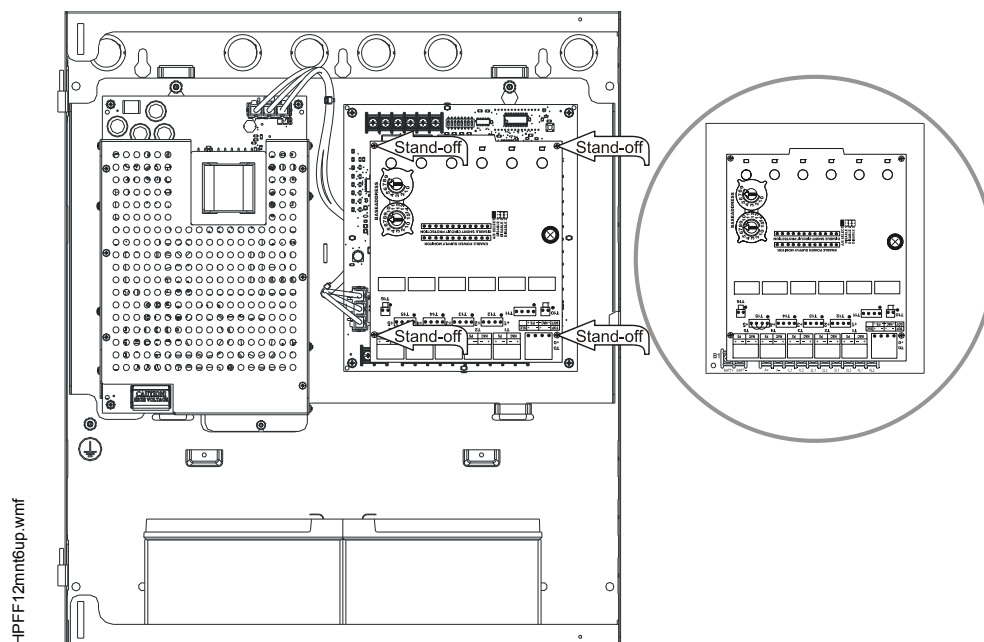
Figure 2.15 Mounting Details for Six-Output Modules from Honeywell Fire System
