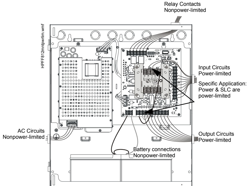
Figure 2.16 Power-Limited Wiring Example: HPFF12(CM)(E) Shown with Single-input Control Module
