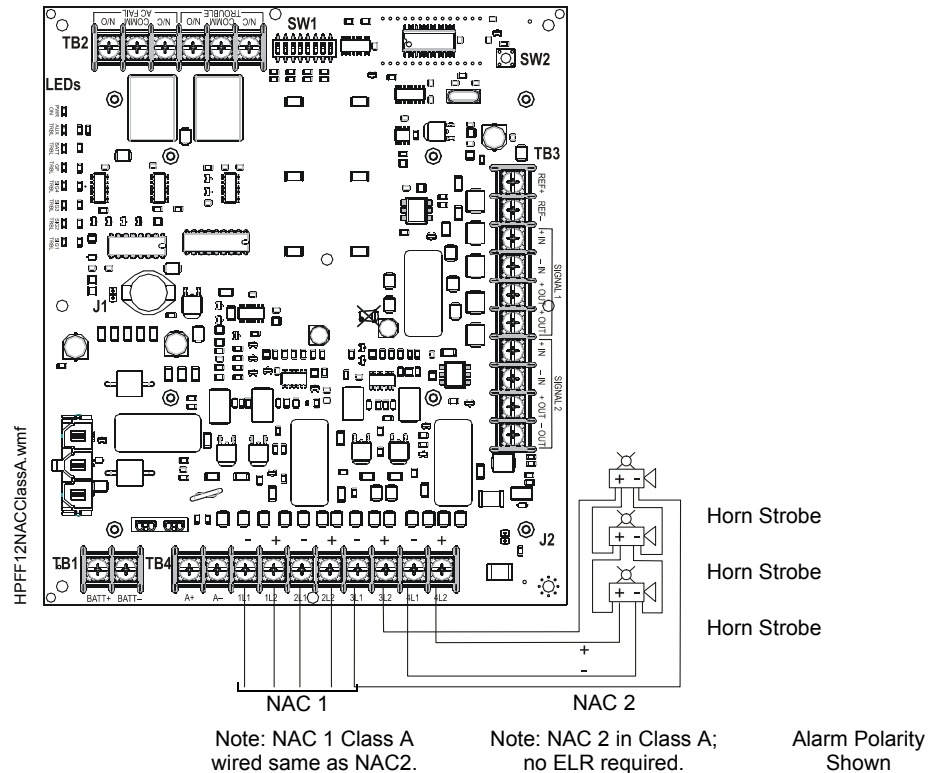
Figure 2.11 Two NACs in Class A (Style Z)
