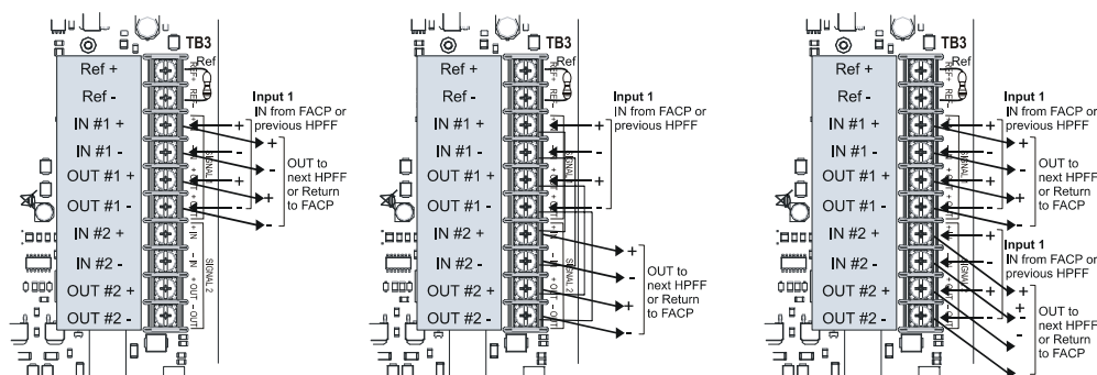
Figure 5.8 Class A Input Connections
