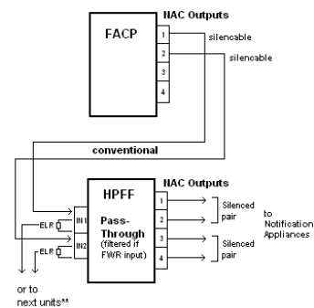
Figure 5.10 Selective Silencing Connections
