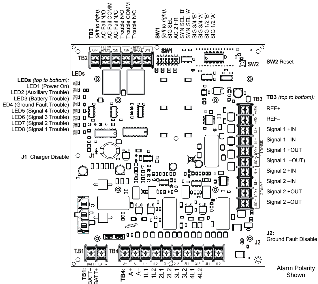
Figure 1.1 Control Circuit Board
