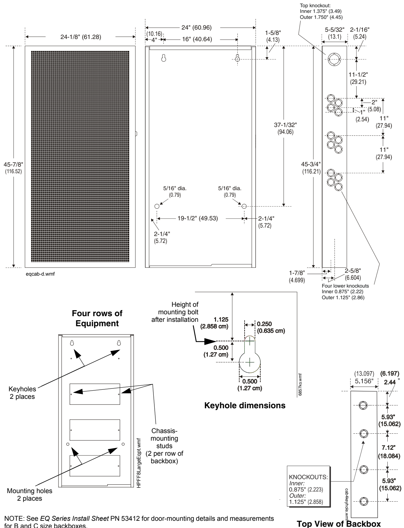
Figure 2.3 FACP Cabinet-Mounting Details: Backbox-Mounting Holes and Chassis-Mounting Studs (EQBB-D4 shown)
