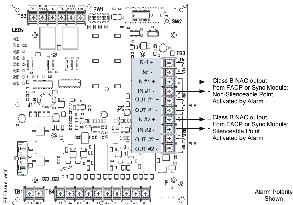
Figure 5.3 Wiring for Selective Silence
