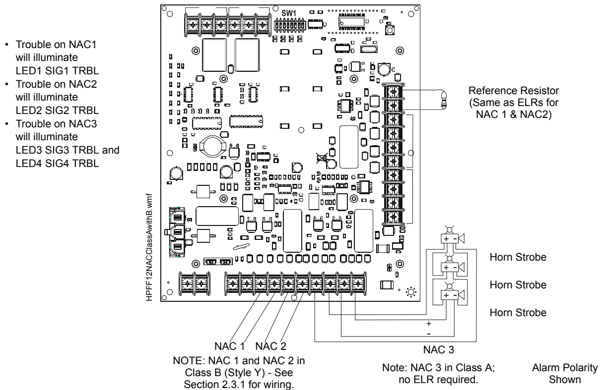
Figure 2.12 Configuring Two Class B NACs and One Class A NAC on One HPFF
