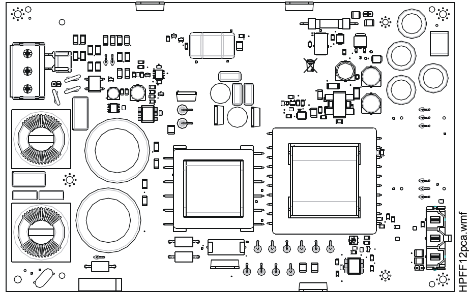
Figure 1.2 HPFF12 24 VDC Power Supply Circuit Board
