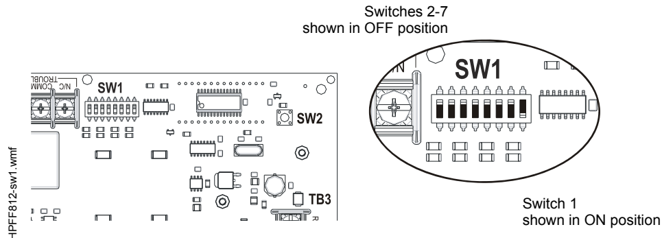
Figure 3.1 Field-Programming DIP Switches
