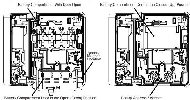
FIGURE 2. BATTERY INSTALLATION
