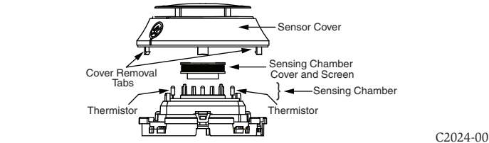
FIGURE 4. CLEANING THE PHOTO/HEAT DETECTOR
