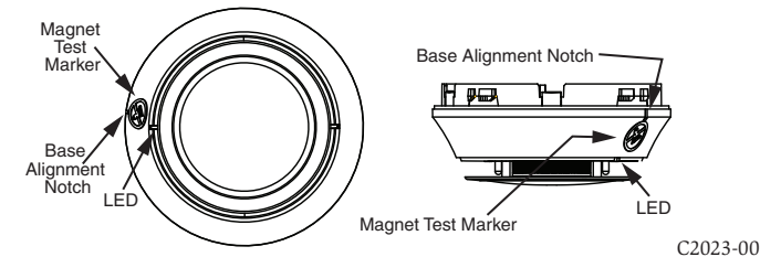
FIGURE 4. CLEANING THE PHOTO/HEAT DETECTOR
