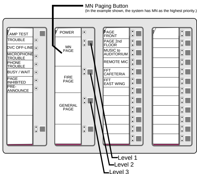
Figure 4.3 DVC-KD Keypad
