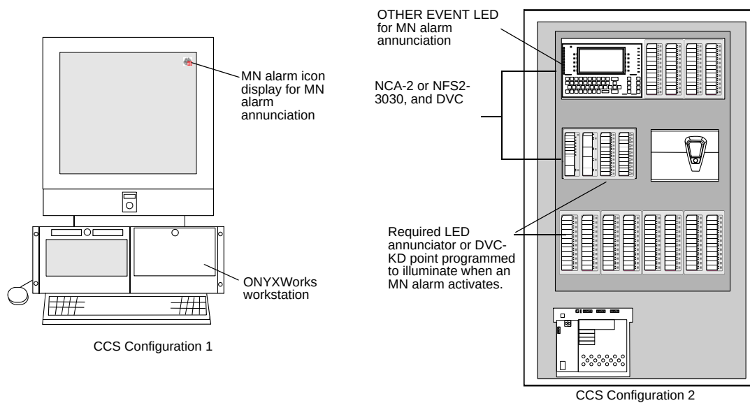
Figure 2.3 CCS Configurations
