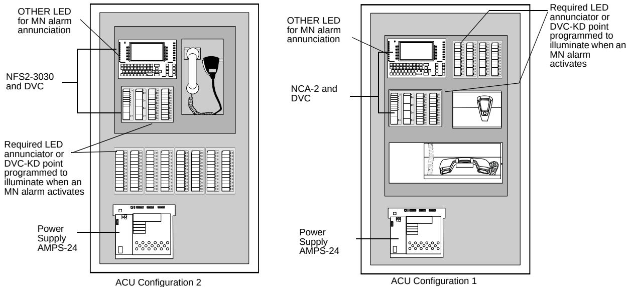
Figure 2.1 ACU Configurations
