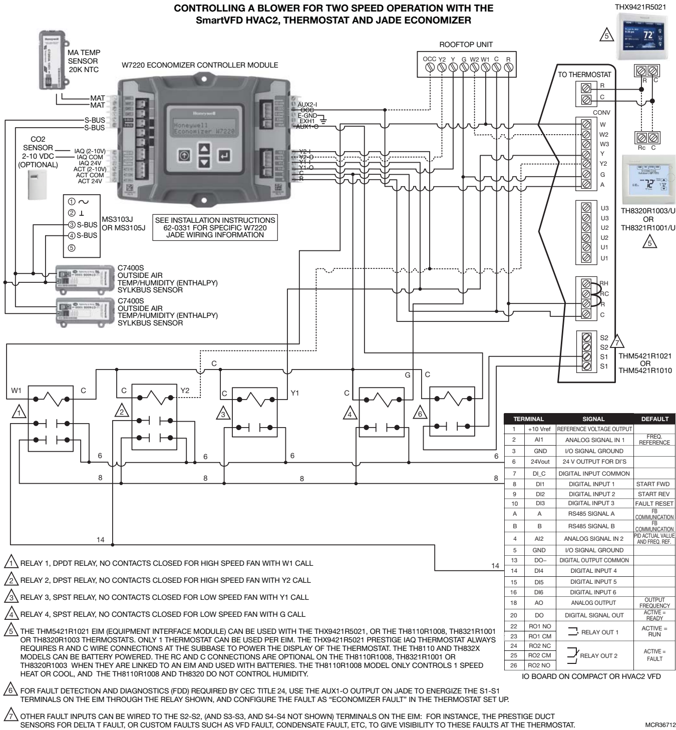
Fig. 3. Figure showing RTU retrofit wiring using the HVFDCDxxxx or HVFD2D SmartVFD Compact or HVAC2 and four relays.
