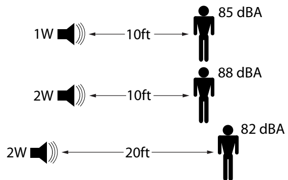
Figure 1. dB Rules of Thumb
