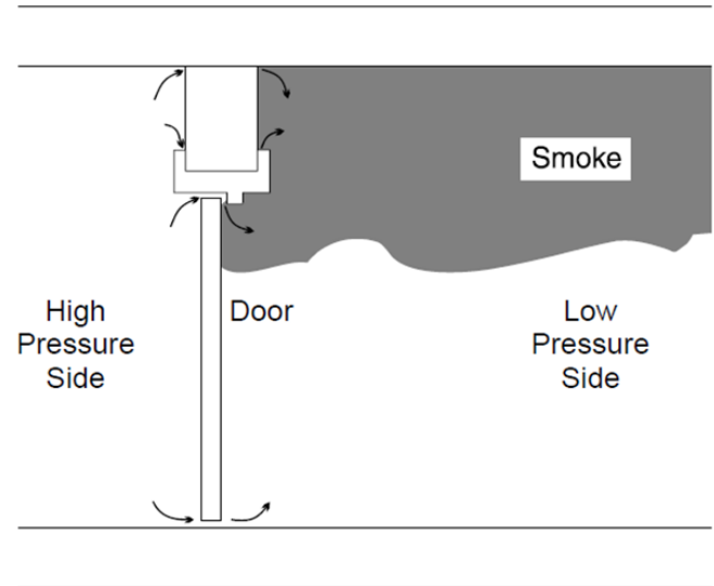
Figure 2.4 Pressurization
